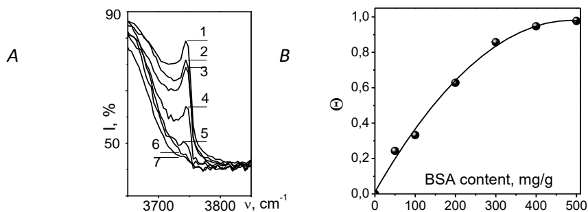
Fig. A - IR spectra of the silica (1) after 50 (2), 100 (3), 200 (4), 300 (5), 400 (6), 500 mg/g (7) BSA adsorption. B - The perturbation degree of OH-groups as a function of BSA content
