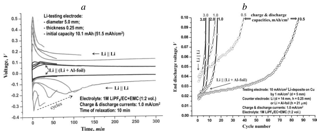
Fig. Electrochemical behavior of Li || Li and Li || (Li+Al-foil) half cells with working electrode prepared from Li-foil (a) and via Li-electroplating (b)
