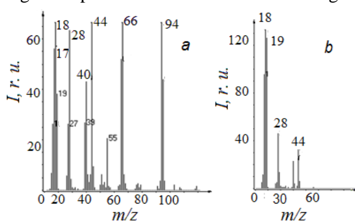
Fig. Mass spectra of low temperature (a) and high temperature (b) structures
