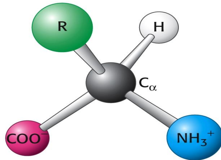
D isomer
