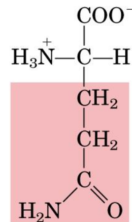
Glutamine
