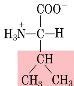
Valine
